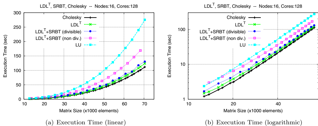
Fig. 9. Problem scaling comparison of LDL^T +SRBT against Cholesky on a 16 \times 8 = 128 core cluster.
